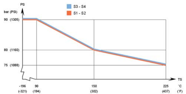
CBXP52 – UL approval pressure/temperature graph
