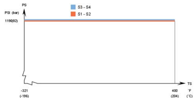
CBXP27 – UL approval pressure/temperature graph
