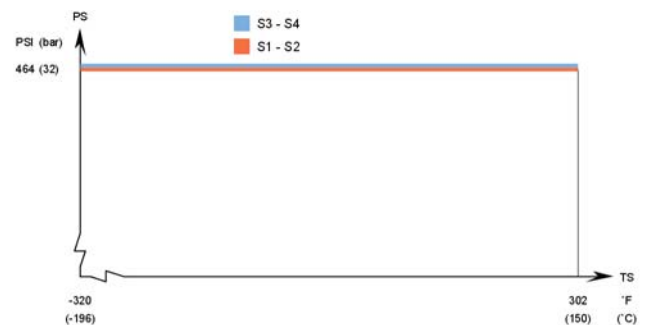
CBH16AQ – UL/CRN approval pressure/temperature graph
