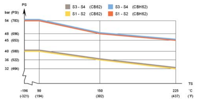
CB62/CBH62 – UL approval pressure/temperature graph
