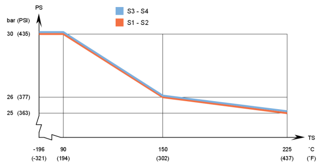
CB110AQ – UL approval pressure/temperature graph
