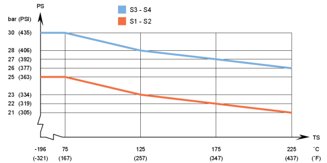
AlfaNova 52AQ - PED approved pressure/temperature graph
