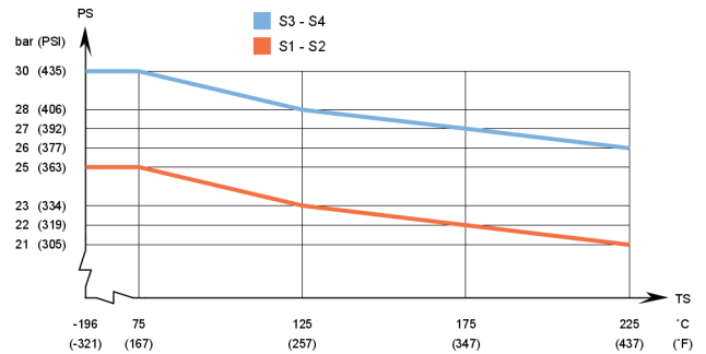
AlfaNova 27AQ - PED approved pressure/temperature graph
